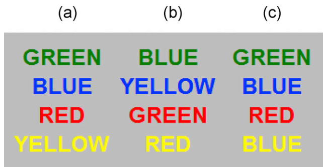
Fig. 2. Examples of (a) congruent, (b) incongruent, and (c) mostly congruent Stroop lists. In each case, the test taker must state the hue in which the words are printed, while ignoring the word itself.
